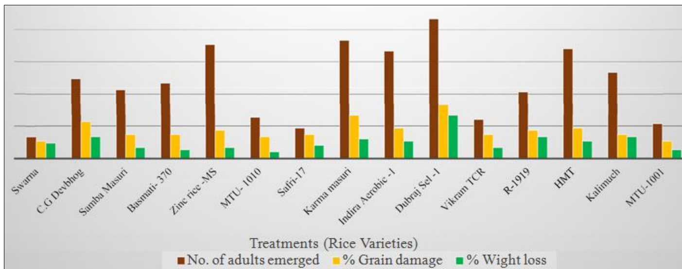
Fig 1: Number of adult emergences, % grain damage and % weight loss in different rice varieties at 60 DAS
